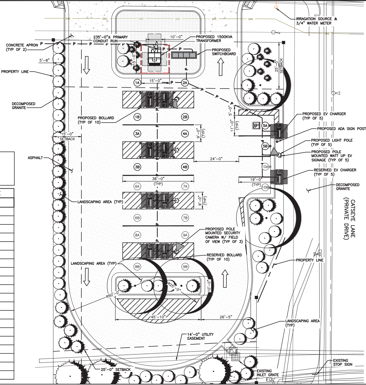
SITE PLAN
